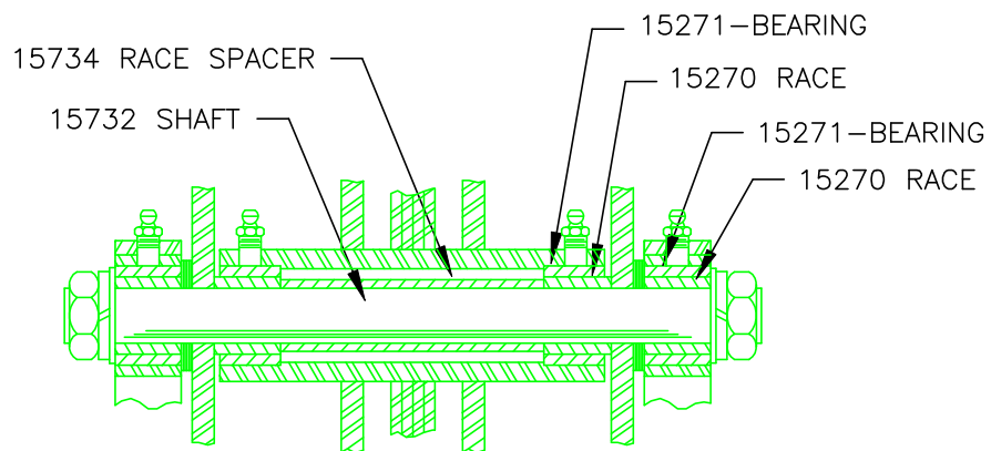
DETAIL "A"
