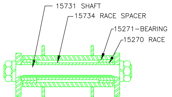
DETAIL "C"
