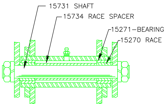
DETAIL "B"
