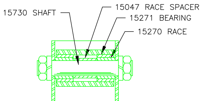
DETAIL "D"
